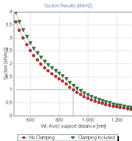
Suction results [kN/m 2 ]
