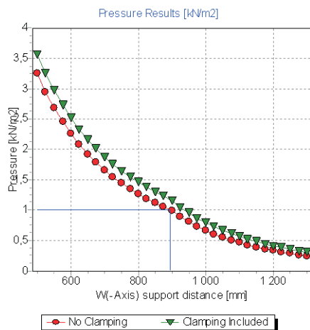
Pressure results [kN/m 2 ]
