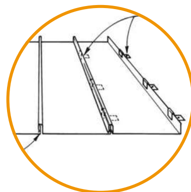
DETAIL UCHYTENIA
